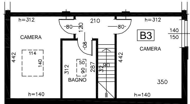
PIANO MANSARDA
